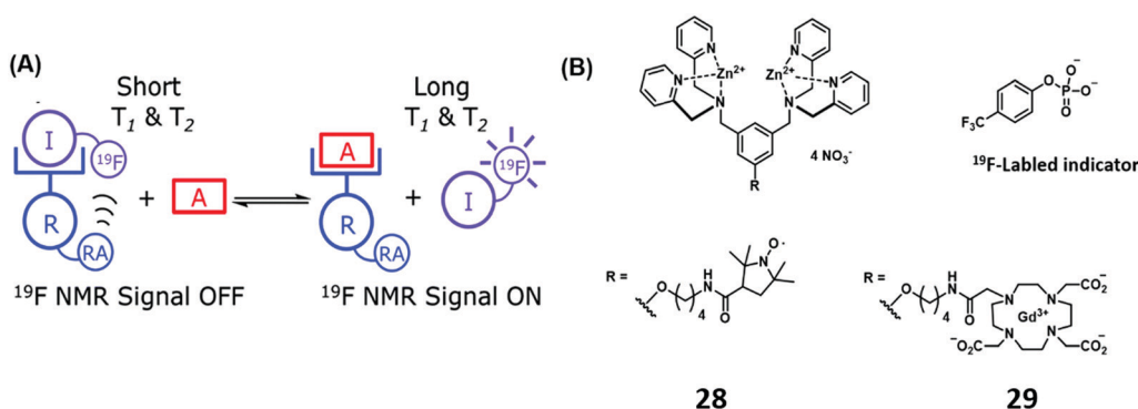
Scheme 17 (a) Basic schematic of a ^{19}\text{F} NMR-based IDA assay for the detection of PPI. (b) \text{Zn(II)} -bis(dipicolylamine) receptor appended with a relaxation agent (RA), a nitroxide motif ( 28 ) and \text{Gd(III)} -DOTA ( 29 ). Reproduced from ref. 27 with permission from [The Royal Society of Chemistry], copyright [2014].
