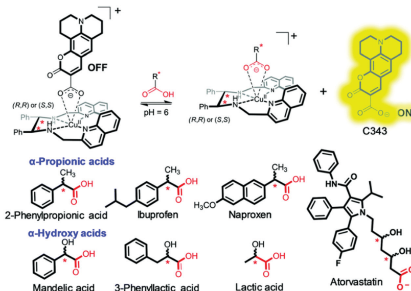
Scheme 9 Chiral copper(II)-based receptors— [Cu^{RR}]^{2+} and [Cu^{SS}]^{2+} that allow the enantiomeric composition of chiral carboxylates, such as ibuprofen, to be determined. Reproduced from ref. 13 with permission from [The Royal Society of Chemistry], copyright [2019].
