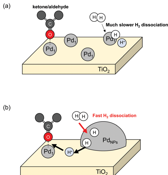
Fig. 2 Schematic image of the ketone/aldehydes hydrogenation over \text{Pd}_1/\text{TiO}_2 (a) and \text{Pd}_{\text{NPs}}/\text{TiO}_2 (b).
