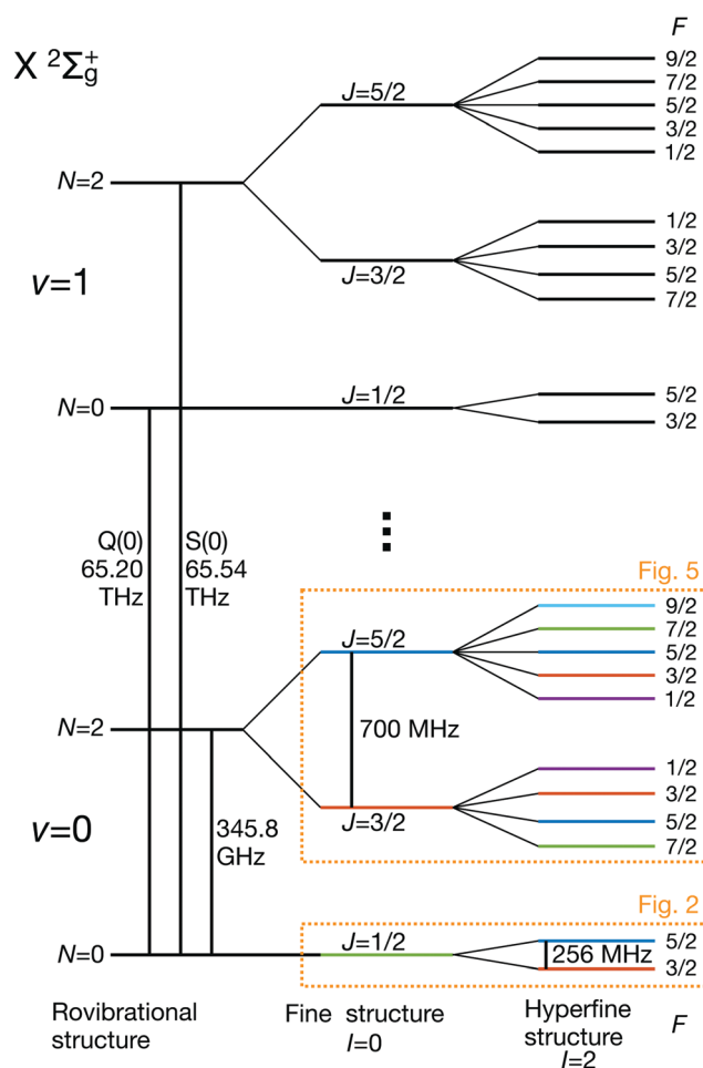
Fig. 1 Partial schematic of the field-free energy levels of \text{N}_2^+ in the electronic ground state, X^2\Sigma_g^+ (not to scale). The states are labeled using the Hund's case ( b, \beta_j ) basis eqn (3). The dotted boxes indicate the level subspaces shown in Fig. 2 and 5 where the relevant Zeeman manifolds are displayed. The color coding of the levels is identical with the one used in these figures.
