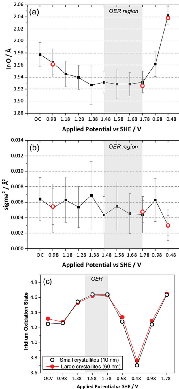
Fig. 4 Plots of EXAFS-derived (a) Ir–O distance, (b) Debye–Waller factor, and (c) comparison of Ir oxidation state from XANES for two particle sizes of (\text{Ca}_{0.70}\text{Na}_{0.24})_2\text{Ir}_2\text{O}_6\cdot\text{H}_2\text{O} showing also recyclability upon a second oxidation sweep. In (a and b) the red circles are repeated measurements from a second electrode on a later experimental run to check reproducibility. OC = open circuit.
