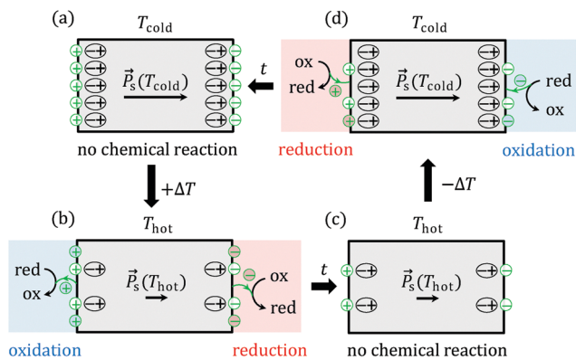
Fig. 2 Simplified model of the pyroelectrocatalytic effect based on externally compensating free (surface) charges (green). (a and c) The charge-balanced pyroelectric at thermal equilibrium in a chemically labile medium. The temperature-induced polarisation change upon (b) heating and (d) cooling generates an electric potential (excess charges are shaded red and blue) able to trigger redox reactions within the medium. ox: oxidised chemical species, red: reduced chemical species. Not included are further screening layers on the surface (e.g. electrical double layer).
