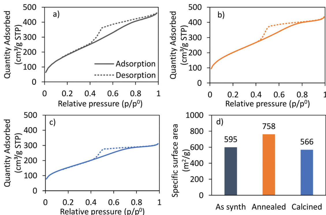
Fig. 2 The \text{N}_2 -adsorption (solid)/-desorption (dashed) isotherms of the (a) as-synthesised, (b) annealed, (c) calcined CoRe-aerogel and (d) the corresponding BET surface areas.
