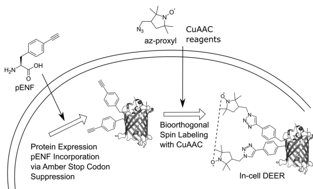
Fig. 1 Schematic overview of the in vivo spin labeling approach via copper-catalyzed [3+2] azide–alkyne cycloaddition followed by in-cell EPR distance determination. The nCAAs pENF is incorporated site-specifically into eGFP using amber stop codon suppression. The eGFP-expressing E. coli cells are subjected to CuAAC-based spin labeling and subsequent, DEER distance determination is performed directly inside the cell.
