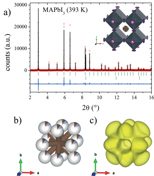
Fig. 6 a) SXRDP profile after Rietveld refinement at 393 K and schematic view of MAPbI 3 (inset) at 393 K in the Pm\bar{3}m space group. b) and c) Detailed views of C/N positions and DFM density, respectively.
