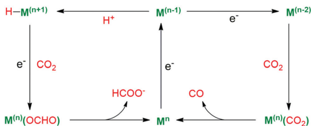
Fig. 13 The competing pathways for CO and \text{HCOOH} formation from \text{CO}_2 .
