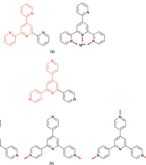
Scheme 2 Examples of tpy motifs as units within quaterpyridines. (a) 4'-(Pyridin-2-yl)-2,2':6',2''-tpy contains a 2,2':4',2''-tpy unit (in red) but typically binds metal ions as a bis(chelate). (b) 4'-(Pyridin-4-yl)-4,2':6',4''-tpy contains a 4,2':4',4''-tpy unit (in red); three possible ditopic modes of bonding of 4'-(pyridin-4-yl)-4,2':6',4''-tpy represented in the CSD by refcode entries AGUPUO (left), QOTREY (middle) and RIGPII (right).
