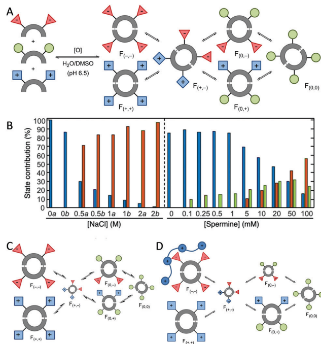
Fig. 3 Use of chemometrics to unravel multi-stimuli response in DCL of macrocyclic pseudopeptides: (A) schematic representation of the DCL generated by disulfide formation in aqueous media giving yield to six different families classified by their charge at neutral pH. (B) Bar plots of the scores of the three states resolved by MCR-ALS analysis of the HPLC in the presence of salt or spermine data sets. (C) Schematic representation of the changes in concentration of the families of macrocycles due to the salt effect (larger/smaller size symbols represent an increase/decrease of the concentration) (D) cartoon representation of the effect of the spermine polycation binding on the DCL.
