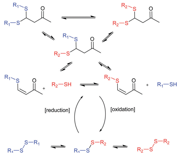
Fig. 4 Antiparallel chemistries described by Otto. 40 The final state of the system between thio-Michael chemistry (top) or disulfide chemistry (bottom) can be switched by addition of reducing or oxidising agents.
