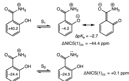
Fig. 3 Computed NICS(1) zz and \Delta\text{NICS}(1)_{zz} (sum of NICS(1) zz values of the conjugate base minus that of the acid) (in ppm) values for the S_0 and S_1 states of protonated salicylamide and its conjugate base at CASSCF(12,12)/6-311+G(d,p). Negative \Delta\text{NICS}(1)_{zz} values indicate antiaromaticity relief upon formation of the excited conjugate base. Positive \Delta\text{NICS}(1)_{zz} values in the ground state indicate aromaticity loss upon formation of the conjugate base. An experimental \Delta pK_a value is included for reference.
