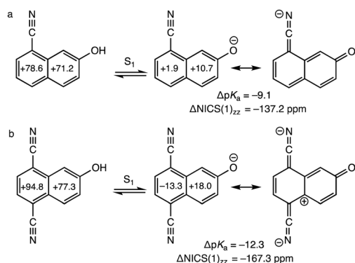
Fig. 2 Computed NICS(1) zz and \Delta\text{NICS}(1)_{zz} (sum of NICS(1) zz values of the conjugate base minus that of the acid) (in ppm) values for the S_1 states of the acid and conjugate base at CASSCF(12,12)/6-311+G(d,p), for (a) 8-cyano-2-naphthol and (b) 5,8-dicyano-2-naphthol. Negative \Delta\text{NICS}(1)_{zz} values indicate antiaromaticity relief upon formation of the excited conjugate base. Experimental \Delta pK_a values are included for reference. Note resonance form showing delocalization of the negative charge into the CN groups.
