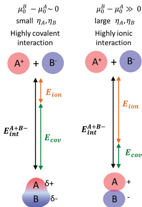
Scheme 7 Effects of chemical strength and hardness of species A and B on the nature of \text{A} + \text{B}^- ion-pair interaction.
