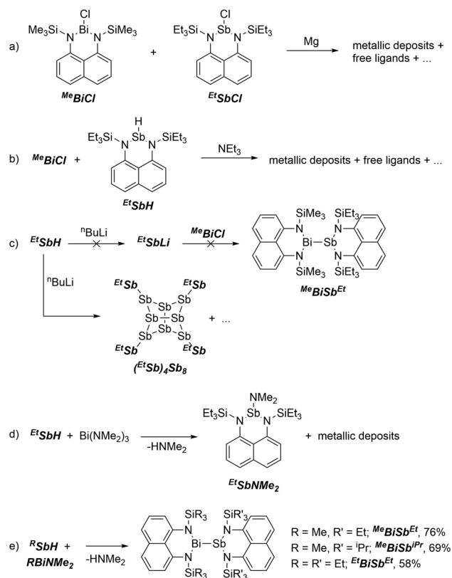
Scheme 2 Synthesis of (\text{EtSb})_4\text{Sb}_8 and derivatives of \text{MeBiSbR}^i .
