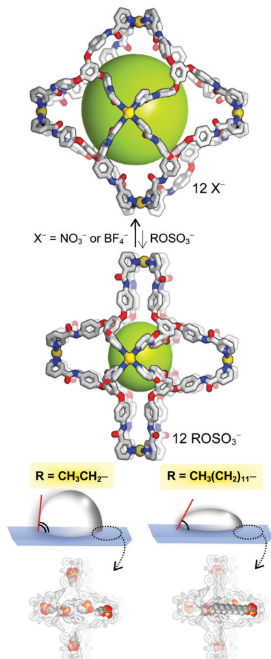
Scheme 1 Encapsulation of \text{ROSO}_3^- ( R = \text{ethyl-}, \text{octyl-}, \text{decyl-}, \text{dodecyl-}, \text{and tetradecyl-} ) within present spherical coordination cages and different surface tensions depending on included alkyl chains of surfactant.
