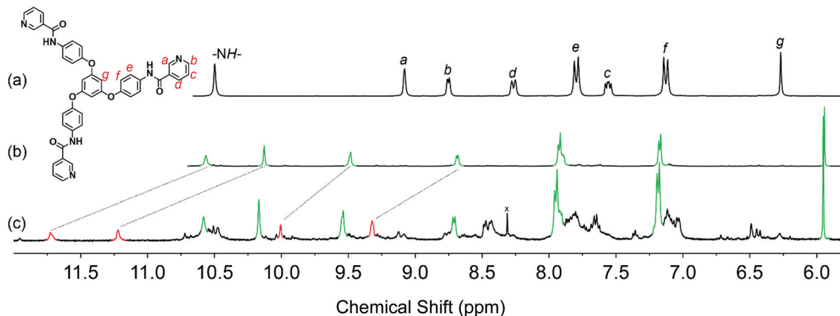
Fig. 2 ^1\text{H} NMR spectra for L (a), \mathbf{1}\cdot\mathbf{12NO}_3 (b), and after addition of 12 equiv. of \text{NaC}_{12}\text{H}_{25}\text{OSO}_3 into \mathbf{1}\cdot\mathbf{12NO}_3 (c) in \text{Me}_2\text{SO}-d_6 . The \mathbf{1}\cdot\mathbf{12NO}_3 and \mathbf{2}\cdot\mathbf{12C}_{12}\text{H}_{25}\text{OSO}_3 resonances are indicated by the green and red signals, respectively.
