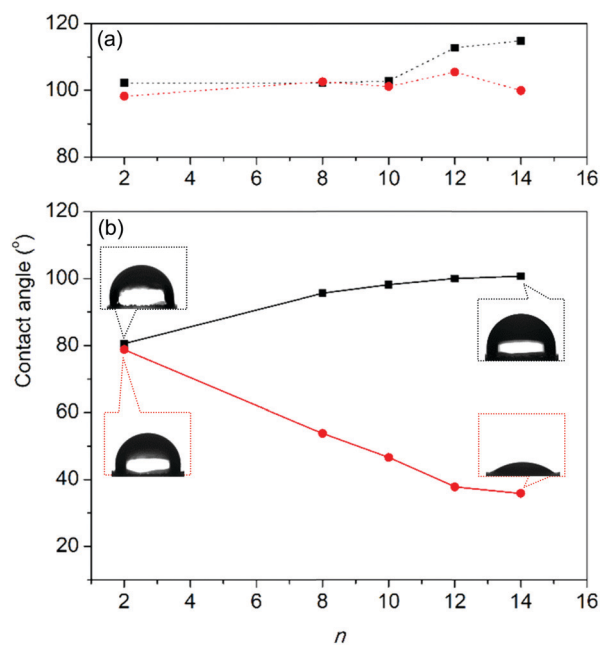
Fig. 3 Surfactant responsive contact angles on fine-ground crystal surface of \mathbf{2}\cdot\mathbf{12C}_n\text{H}_{2n+1}\text{OSO}_3 at 0 min (a) and after 10 min (b) (black line: drop of \text{H}_2\text{O} ; red line: mixture solution of water and ethanol (4:1)).
