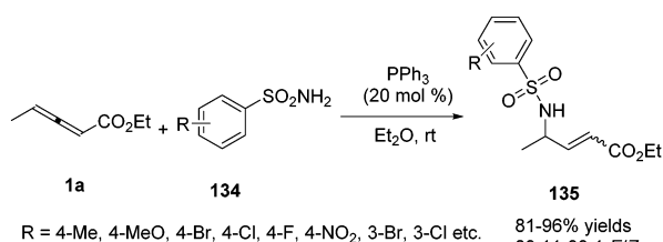
Scheme 43 Phosphine-catalysed \gamma -umpolung additions of sulphonamides to \gamma -substituted allenates.
