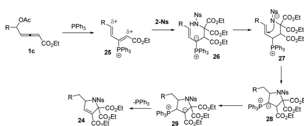
Scheme 8 Plausible mechanisms.
