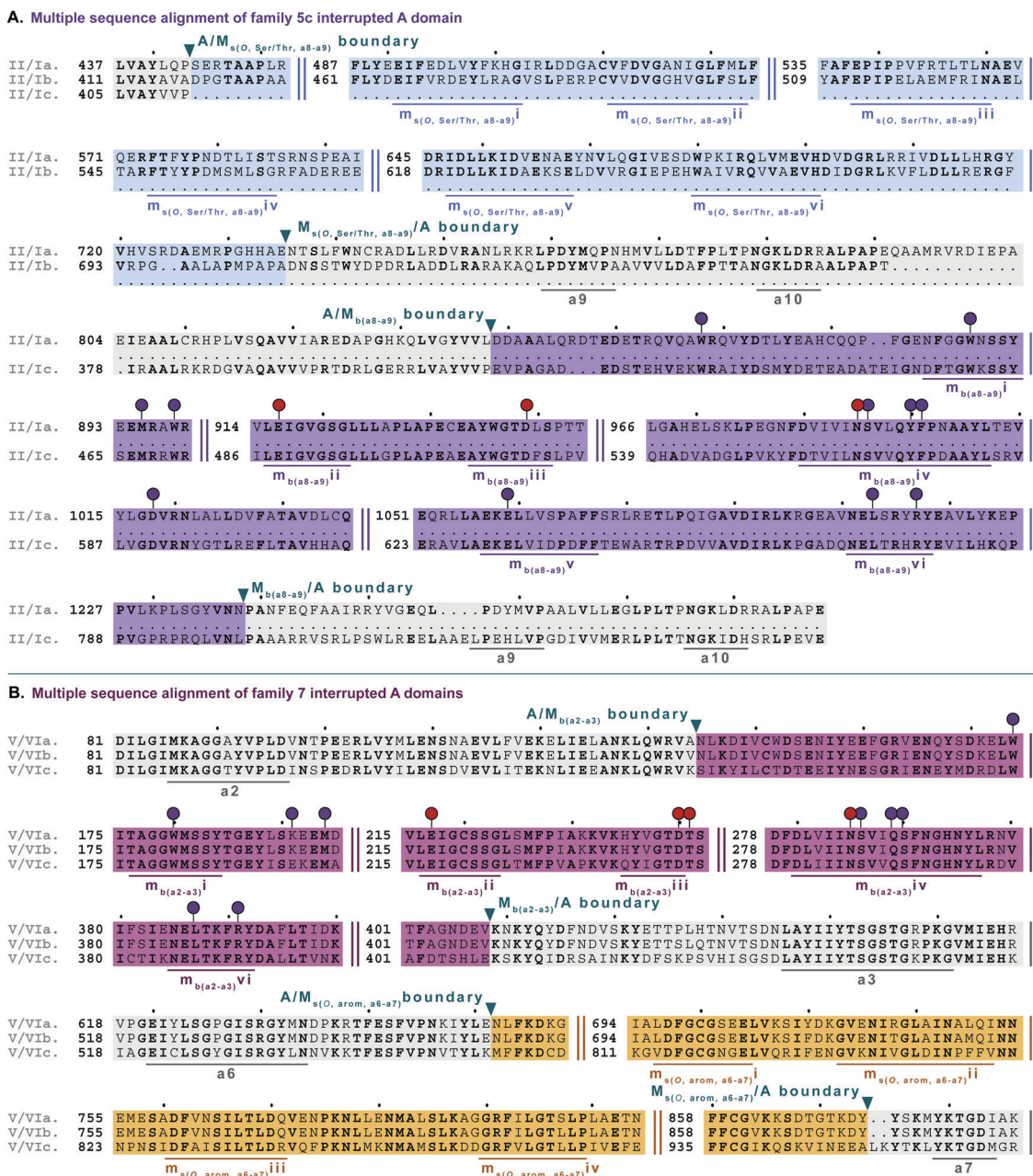
Fig. 10 Multiple sequence alignments of (A) family 5c interrupted A domain (sequence "a") alignment with representative type II and type I M domains, KtzH( M_{II} ) 4 (sequence "b") and TiO 2 ( M_I ) 4 (sequence "c"), respectively, and (B) family 7 interrupted A domains. The A domain is highlighted in light grey and conserved A domain motifs are underlined in dark grey. The M_{II} is highlighted in light blue and the conserved motifs are underlined in dark blue. The M_I is highlighted in light purple, and the conserved motifs are underlined in dark purple. The red and dark purple balloons in panel A correspond to residues involved in SAM and amino acid bound Ppant arm binding, respectively, according to the structure of TiO 2 ( A_8M_I A_9 ) 4 . 14 The identical corresponding residues in type V M domain are also indicated in the same way. Type V M domain is highlighted in light pink and the conserved motifs are underlined in dark pink. Type VI M domain portion is highlighted in light orange and the conserved M domain motifs are underlined in dark orange. The boundaries between the domains are indicated by a triangle. Breaks in the sequences are indicated by two parallel bars. The full sequence alignments and accession numbers are presented in Fig. S19 and S21 (ESI†).
