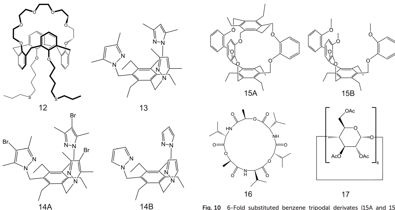
Fig. 9 Calix[4]arene-crown-6 ( 12 ) functionalized with alkyl sulfide units reported in the work of Saiapina and co-workers. 93 The 6-fold substituted benzene tripodal derivatives, reported in the works of Chin et al. ( 13 ; 80 14A and 14B 95 ), as \text{NH}_4^+ ionophores.
