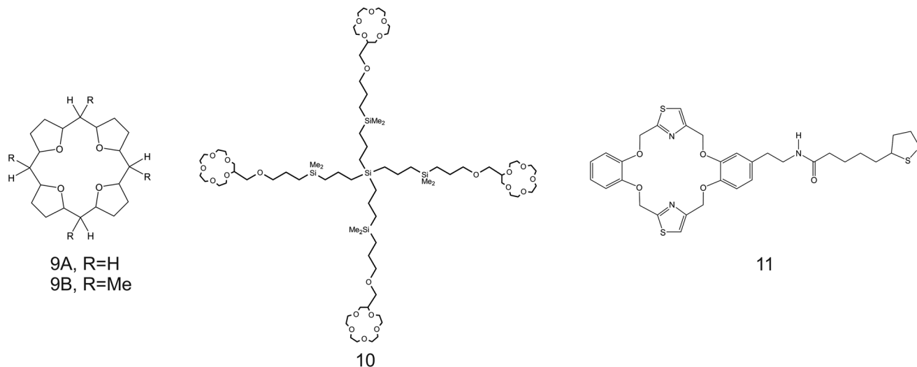
Fig. 8 THF-containing 16-crown-4 derivative ( 9A and 9B ), 15-crown-5 substituted carbosilane dendrimer ( 10 ), and DB18C6 ( 11 ) reported in the works of Jin et al. , 90 Chandra et al. , 91 and Jin et al. , 92 respectively, as \text{NH}_4^+ ionophores.
