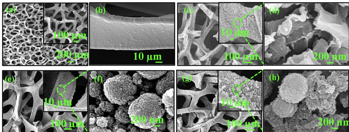
Fig. 2 FESEM images at different magnifications of (a) and (b) bare NF, (c) and (d) PANI, (e) and (f) CaMoO 4 , and (g) and (h) CaMoO 4 /PANI.
