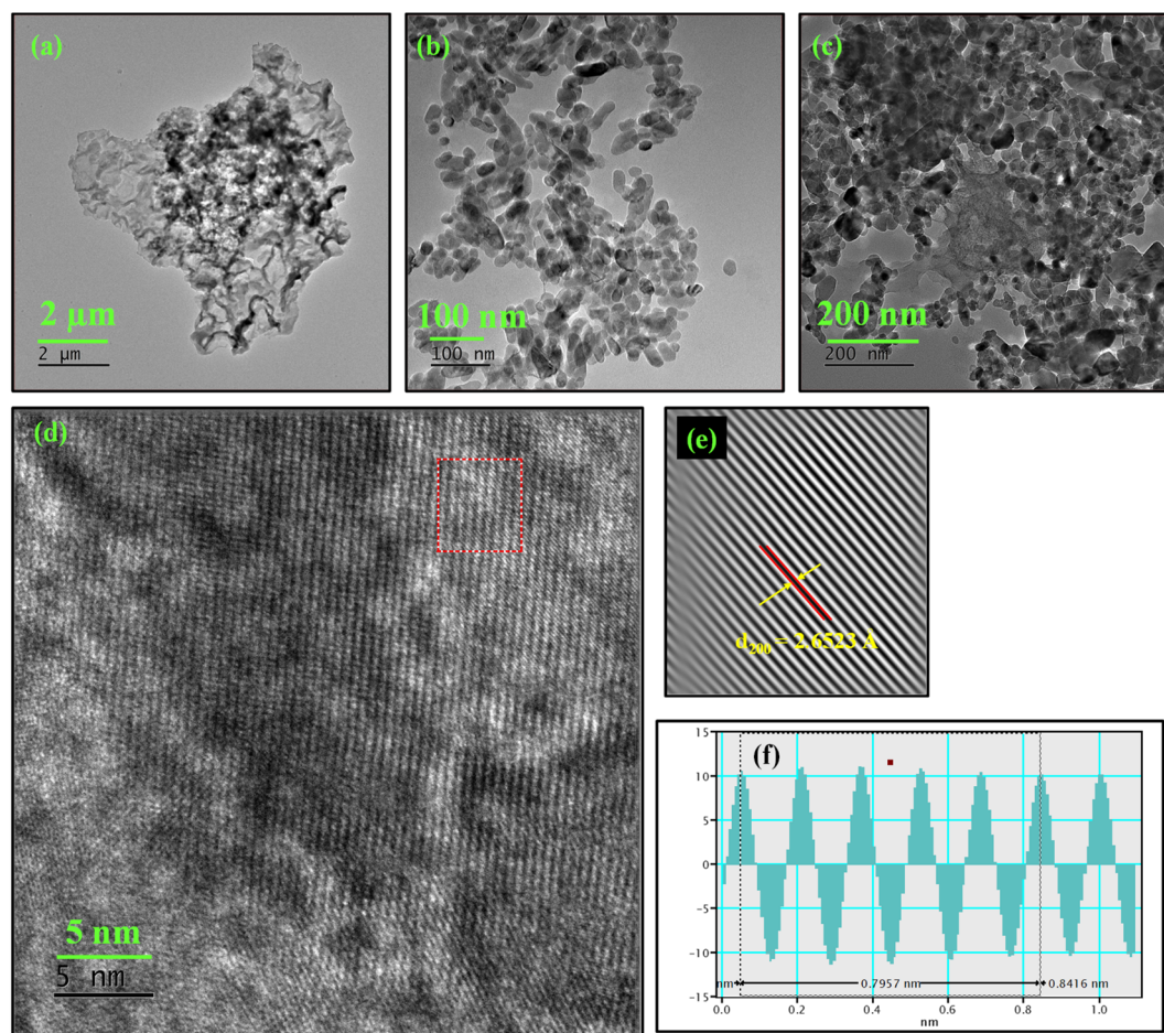
Fig. 3 TEM images of (a) PANI, (b) CaMoO 4 , (c) CaMoO 4 /PANI, (d) HRTEM of CaMoO 4 /PANI, (e) IFFT and (f) profile of IFFT CaMoO 4 /PANI.
