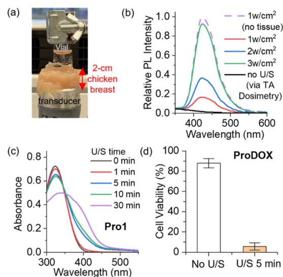
Fig. 5 (a) A photograph showing our setup applying LITUS through a 2 cm thick chicken breast tissue to a solution. (b) Fluorescence spectra of 20 mM TA solutions after 5 min of LITUS irradiation at varied sound intensity (1 MHz, 50% duty cycle) applied through chicken breast. All traces are normalized relative to the fluorescence of a TA solution sonicated ( 1 \text{ W cm}^{-2} , 5 min) without chicken breast (dashed line). (c) Absorption spectra monitoring the release of 4-nitroaniline from a 50 \mu\text{M} Pro1 solution as a function of sonication ( 3 \text{ W cm}^{-2} , through chicken breast). (d) MTT viability assay with HeLa cells show LITUS-induced ( 3 \text{ W cm}^{-2} , through chicken breast) cytotoxicity of ProDOX .
