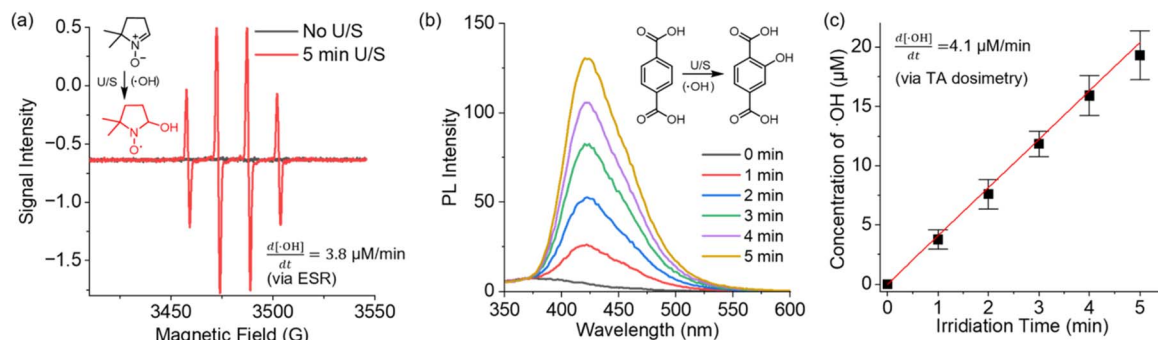
Fig. 2 (a) ESR spectra of a 5 mM solution of DMPO in PBS before and after sonication. (b) Sonochemical conversion of TA (20 mM in PBS) to hTA monitored by fluorescence spectroscopy. (c) Concentration of sonochemical \cdot\text{OH} as a function of sonication time, calculated by multiplying the concentration of hTA by 1/0.35.
