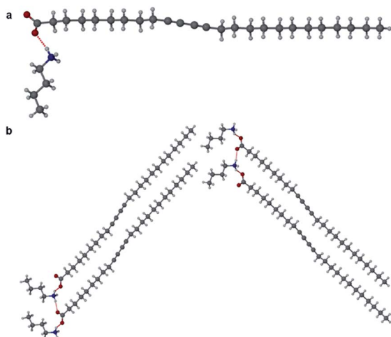
Fig. 8 (a) The X-ray structure of 1 · 8 (b) in the (100) crystallographic plane.
