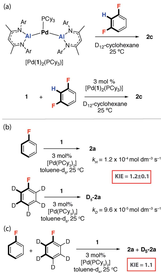
Fig. 3 (a) [Pd( 1 ) 2 (PCy 3 )] as a catalyst for C–F alumination of 1,3-diFB. (b) KIE in the reaction of FB with 1 through measurement of k obs and (c) an intermolecular competition experiment.
