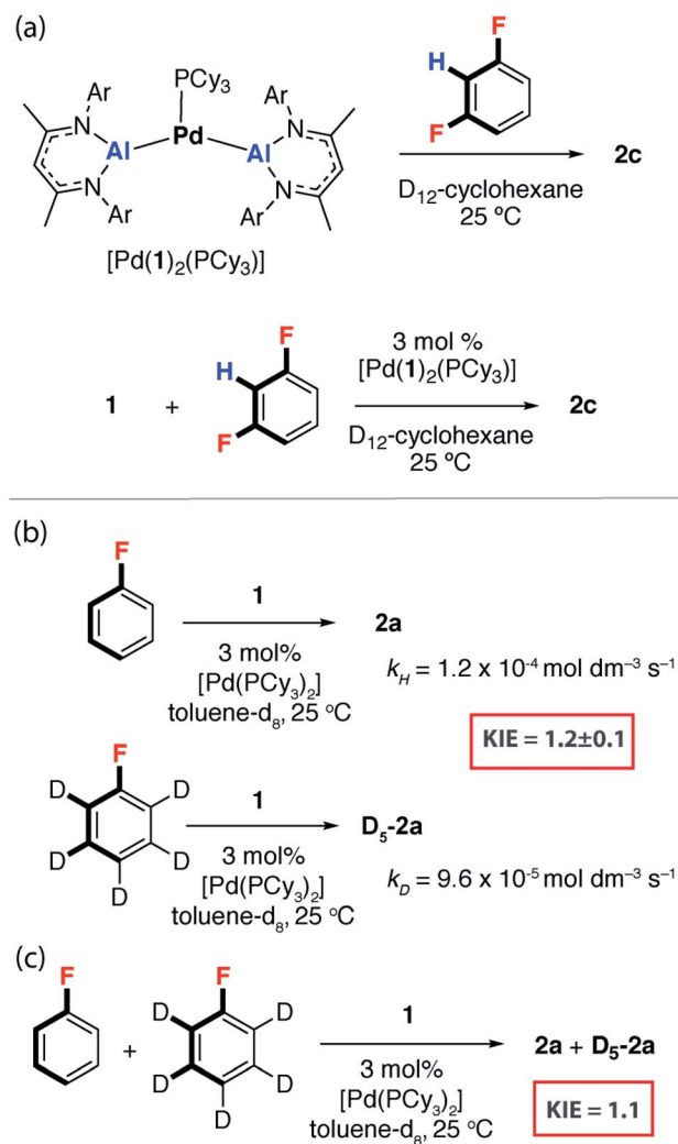
Fig. 3 (a) [Pd( 1 ) 2 (PCy 3 )] as a catalyst for C–F alumination of 1,3-diFB. (b) KIE in the reaction of FB with 1 through measurement of k obs and (c) an intermolecular competition experiment.
