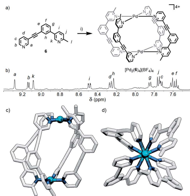
Fig. 6 (a) Formation of the cis\text{-Pd}_2\text{L}_4 cage [\text{Pd}_2(6)_4](\text{BF}_4)_4 . Reagents and conditions: (i) [\text{Pd}(\text{CH}_3\text{CN})_4](\text{BF}_4)_2 , d_6\text{-DMSO} , rt, 24 h. (b) Partial 1 H NMR spectrum (400 MHz, 298 K, d_6\text{-DMSO} ) of [\text{Pd}_2(6)_4](\text{BF}_4)_4 . Calculated structure (B3LYP/6-31G(d)/SDD) of cis\text{-}[\text{Pd}_2(6)_4]^{4+} viewed from (c) the side, and (d) down the Pd-Pd axis; hydrogen atoms have been omitted for clarity.
