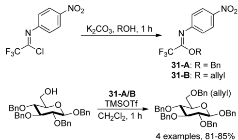
Scheme 31 Synthesis of N -aryl trifluoroacetimidate-based benzyl and allyl protecting group reagents.
