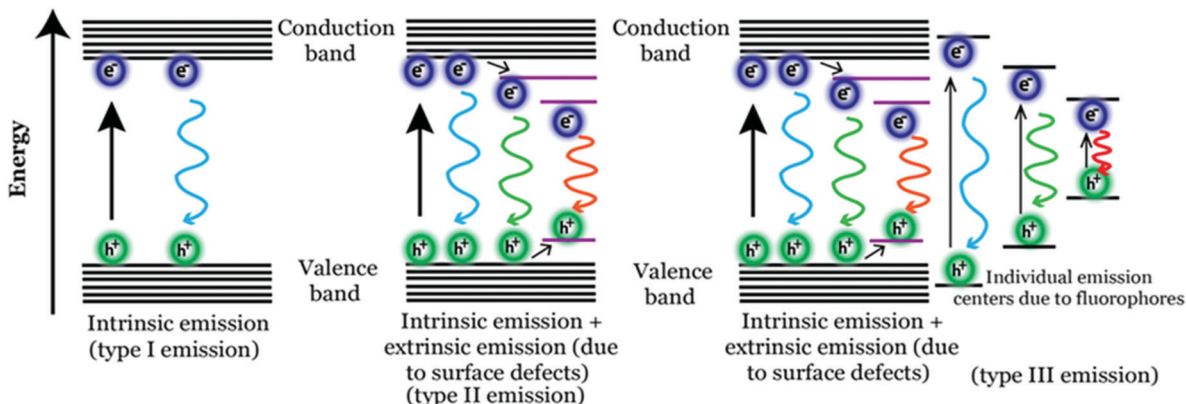
Fig. 4 Schematic representation corresponding to the emission mechanism in Cdote systems.
