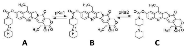
Fig. 1 Structure of the irinotecan molecule in the dicationic (A), monocationic (B) and neutral (C) form, with respect to pK_a values.
