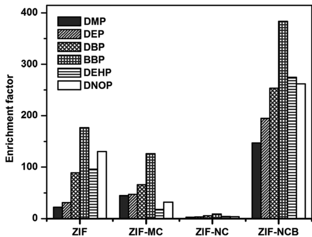
Fig. 7 Enrichment factors obtained for a mixture of six phthalate esters after solvent-assisted extraction using ZIF-8 crystals of different size.
