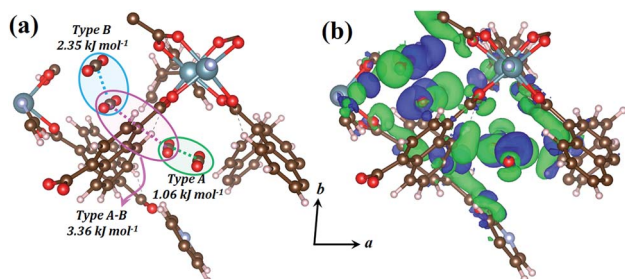
Fig. 7 (a) Perspective view showing CO 2 positions within the geometry-optimised structure of 1 lp with guest–guest interaction energies between different combinations of two CO 2 molecules. (b) EDDM showing areas of enhanced (green) and depleted (blue) electron density of the geometry-optimised structure of 1 lp with respect to its isolated MOF and CO 2 components. The EDDM was generated for a periodic 1 \times 1 \times 1 unit cell and only a fragment is shown for clarity.
