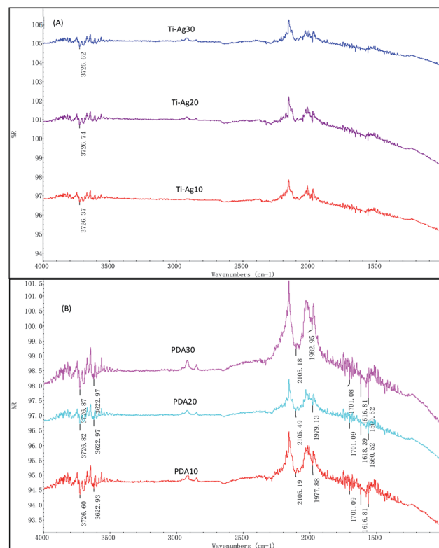
Fig. 5 FTIR spectra of the prepared samples: (A) Ti-Ag, (B) PDA samples.
