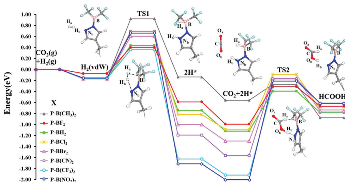
Fig. 23 Potential energy profiles (0 K, no ZPE correction) for \text{CO}_2 hydrogenation in UiO-66-X. Key structures are shown in the diagram for the \text{P-B}(\text{CF}_3)_2 functional group as examples. Figure reproduced from ref. 322 with permission from the American Chemical Society, copyright 2015.
