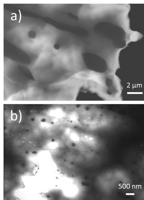
Fig. 2 (a) STEM dark field image of water-quenched and (b) TEM-BF image of MS/SPS (\text{CoGe}_2)_{0.2}(\text{GeTe})_{17}\text{Sb}_2\text{Te}_3 after thermal treatment (3 cycles up to 500 \text{ }^\circ\text{C} ): cobalt germanides ( \text{CoGe}_2 and \text{Co}_5\text{Ge}_7 ; black spots) in (\text{GeTe})_{17}\text{Sb}_2\text{Te}_3 matrix. Note that the precipitates in TEM-BF image appear dark as they are thicker than the surrounding GST matrix, which is caused by Ar-ion-thinning.
