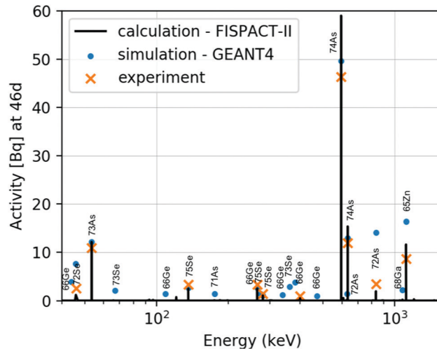
Fig. 4 Comparison of experimentally realized and computationally predicted GaAs gamma decay activity spectra resulting from 63 MeV proton irradiation with 7.5 \times 10^{12} p + per cm 2 (associated with a device dose of 1 Mrad(Si) normal incidence proton beam) at 46 days post-irradiation. These results are used to validate the use of FISPACT-II in computing elemental impurity concentrations as a function of time in orbit.
