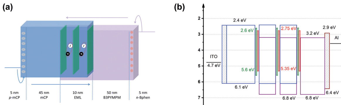
Fig. 2 (a) Device architecture for monochrome OLEDs. Three UN-EMLs (0.1 nm) are spaced by 5 nm mCP : B3PYMPM (1 : 1), which is adopted as a charge recombination layer. The triplet energy of B3PYMPM, mCP and the CT-host blend of mCP:B3PYMPM is 2.68, 2.90 and 2.97 eV, respectively, ensuring efficient triplet confinement. 15 (b) Energy level diagram of the materials used for the device. The highest occupied molecular orbital (HOMO) differences for mCP and Ir(ppy) 2 (acac) and mCP and Ir(MDQ) 2 (acac) are 0.5 eV and 0.75 eV, respectively. 3,15
