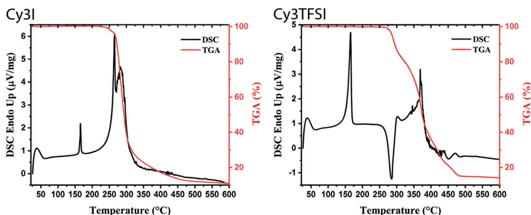
Fig. 2 Dynamic TGA ( 10\text{ °C min}^{-1} ) with the corresponding DSC signal of starting material (Cy3I) and Cy3TFSI.
