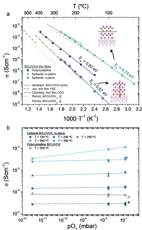
Fig. 3 (a) Arrhenius representation of the evolution of ionic conductivity for different BICUVOX (polycrystalline, epitaxial) films with temperature, all deposited at p = 0.267 mbar. References for bulk polycrystalline BICUVOX, 28 single crystal BICUVOX (parallel and perpendicular to the (100) BICUVOX planes), 48 YSZ thin film 16,46 and CGO thin film 44,45 are included for comparison. Inset schematics show the direction of oxygen mobility in the two measuring configurations, for the epitaxial films. Activation energies ( E_a ) are also indicated for the measured films. (b) p\text{O}_2 dependence of BICUVOX in-plane conductivity, measured in an epitaxial film at different temperatures ( T = 150 – 350 °C) and in a polycrystalline sample at T = 250 °C. Oxygen partial pressure is measured by an oxygen sensor at the outlet of the gases. Dashed lines are included as guide for the eyes.
