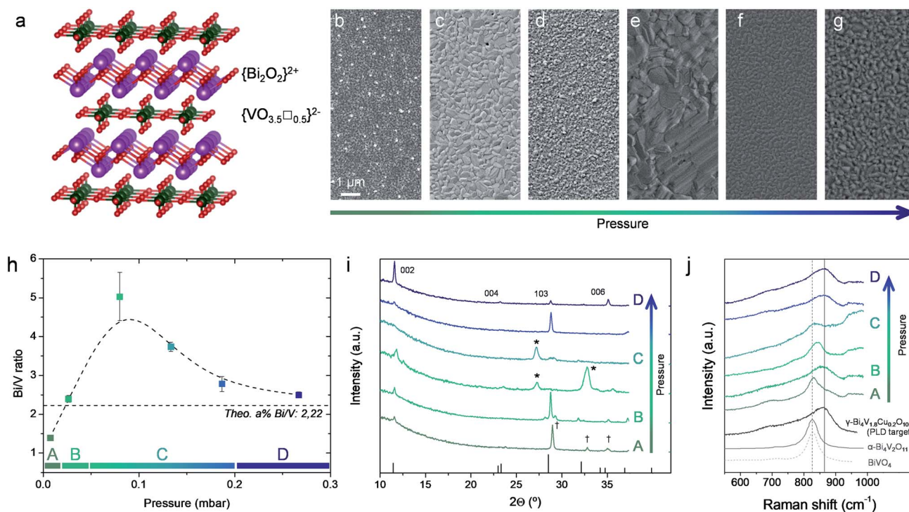
Fig. 1 (a) Atomic representation of the \gamma\text{-Bi}_4\text{V}_2\text{O}_{11} aurivillius layered structure (drawings produced by VESTA 3 software). 50 (b–g) Top view SEM images of representative films deposited by PLD at different background pressures ( p = 0.0067\text{--}0.267 mbar) and a constant target-to-substrate distance of 11 cm, on top of Si substrates. (h) Bi/V ratio as a function of deposition pressure. Dashed line is included as guide for the eyes. Four different pressure regions are identified (A–D) (i) X-ray diffractogram obtained for the same BICUVOX film series. Main diffractions of the \gamma\text{-Bi}_4\text{V}_2\text{O}_{11} phase are indicated (ICDD reference code 00-048-0273), as well as the appearance of secondary phases ( \text{Bi}_2\text{O}_3 *, \text{BiVO}_4 †) (j) Raman spectra of the BICUVOX film series, plus references for \gamma\text{-Bi}_4\text{V}_{1.8}\text{Cu}_{0.2}\text{O}_{10.7} (measured on the pellet used as PLD target), 42 \alpha\text{-Bi}_4\text{V}_2\text{O}_{11} (ref. 43) and \text{BiVO}_4 . 41
