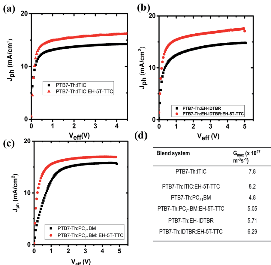
Fig. 8 Comparison of photocurrent J_{\text{ph}} vs. V_{\text{eff}} for binary and ternary blends of (a) PTB7-Th:ITIC, (b) PTB7-Th:EH-IDTBR and (c) PTB7-Th:PC 71 BM, and (d) G_{\text{max}} values for all the blends.
