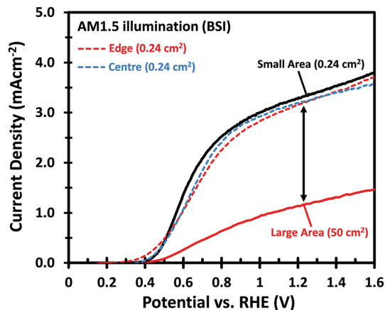
Fig. 1 The current density–voltage ( J – V ) curves of a small area (1 × 2 cm 2 ) W:BiVO 4 photoanode with an illuminated area of 0.24 cm 2 (black), compared to the large area (7 × 12 cm 2 ) W:BiVO 4 photoanode with an illuminated area of 50 cm 2 (red). The dashed curves show the J – V plots from the small W:BiVO 4 pieces (1 × 2 cm 2 ) cut from the centre and edge of the 50 cm 2 sample, with an illuminated area of 0.24 cm 2 . The electrolyte consists of 0.5 M Na 2 SO 3 and 0.1 M KP i buffer in deionized water with pH of 7. BSI: back-side illuminated.
