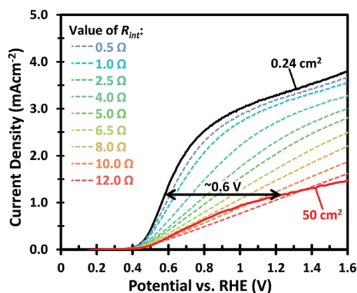
Fig. 2 The J – V curves of small (solid black) and large (solid red) W:BiVO 4 photoanodes measured in 0.5 M Na 2 SO 3 + 0.1 M KP i pH 7 buffer under AM 1.5G illumination. These curves are compared with the calculated J – V curves of a 50 cm 2 W:BiVO 4 photoanode (dashed lines) with the same performance as the small area sample, but subjected to different resistances from 0.5 to 12 Ω.
