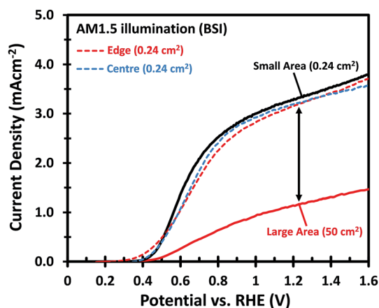
Fig. 1 The current density–voltage ( J – V ) curves of a small area ( 1 \times 2 cm 2 ) W:BiVO 4 photoanode with an illuminated area of 0.24 cm 2 (black), compared to the large area ( 7 \times 12 cm 2 ) W:BiVO 4 photoanode with an illuminated area of 50 cm 2 (red). The dashed curves show the J – V plots from the small W:BiVO 4 pieces ( 1 \times 2 cm 2 ) cut from the centre and edge of the 50 cm 2 sample, with an illuminated area of 0.24 cm 2 . The electrolyte consists of 0.5 M Na 2 SO 3 and 0.1 M KP i buffer in deionized water with pH of 7. BSI: back-side illuminated.
