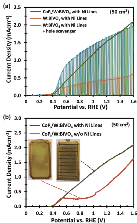
Fig. 5 (a) J - V curves under constant, dark and chopped AM 1.5G illumination comparing the performance of large area ( 50 \text{ cm}^2 ) W:BiVO 4 photoanodes with Ni lines, either in 2.0 M KP i buffer solution with 0.5 M Na 2 SO 3 (blue), or without hole scavenger, before (orange) and after (green) photo-electrodeposition of CoP i . (b) J - V curves comparing CoP i -modified W:BiVO 4 photoanodes with (green) and without (red) Ni lines measured in 2.0 M KP i buffer, pH 7, under AM 1.5G illumination. Inset: photographs of the CoP i deposited on W:BiVO 4 photoanodes without (left) and with (right) Ni lines.
