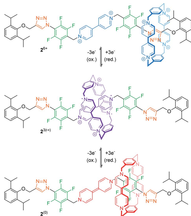
Fig. 3 Tristable [2]rotaxane 2 6+ in its three different redox-states and resulting co-conformations. The unusual CBPQT (0) /tetrafluorobenzene charge-transfer complex is stabilized by the mechanical bond.
