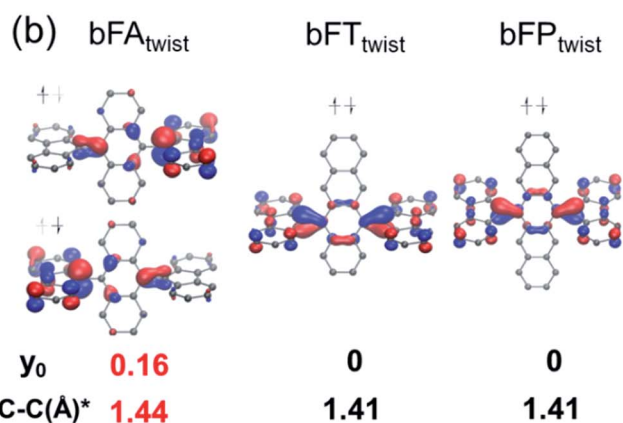
Fig. 5 (a) Energy diagram of \mathbf{bFA} with rotation of the fluorene moiety; (b) HOMOs of the fluorene twisted structure of \mathbf{bFA} ( \mathbf{bFA}_{\text{twist}} ), \mathbf{bFT} ( \mathbf{bFT}_{\text{twist}} ), and \mathbf{bFP} ( \mathbf{bFP}_{\text{twist}} ), with the y_0 value and bond length (*) of the C–C bond between fluorene and acenes.
