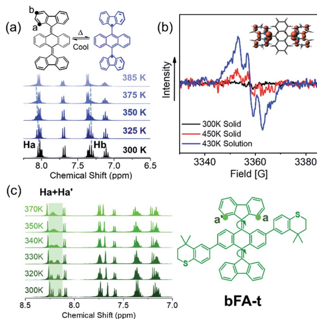
Fig. 4 (a) VT- 1 H NMR of bFA in tetrachloroethane-d 2 ; (b) EPR data of bFA in the solid state at 300 K (black) and 450 K (red) and in dichlorobenzene (4 x 10 -2 M) at 430 K (blue); inset: spin density illustration of the T 1 state of bFA twist (twisted configuration) at the UMO6L/6-311G** level of theory; (c) VT- 1 H NMR of bFA-t and the molecular structure of bFA-t.
