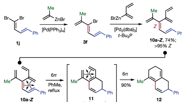
Scheme 3 The first stereoselective synthesis of a [4]dendralene and an unprecedented triene-transmissive twofold 6\pi -electrocyclization sequence.
