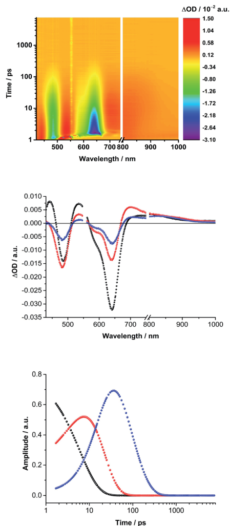
Fig. 6 (Top) Differential absorption spectra obtained by femtosecond transient absorption pump-probe experiments (550 nm, 400 nJ) of (\text{TCBD-aniline})_3\text{-SubPc-(TCBD-aniline)} 2 ( 3 \times 10^{-5} M) in argon-saturated anisole with several time delays between 1 to 7500 ps. (Middle) Deconvoluted evolution associated spectra and (bottom) associated time-dependent amplitudes obtained via global analysis in GloTarAn monitoring formation and decay kinetics.
