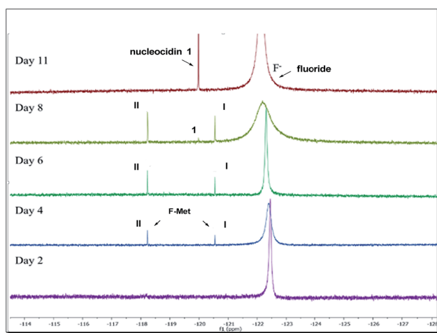
Fig. 2 ^{19}\text{F} -NMR time course of nucleocidin 1 production in S. calvus showing the appearance and disappearance of F-Mets I and II over 11 days.
