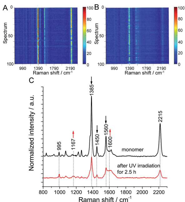
Fig. 3 Waterfall plot of all TERS spectra from maps of a monomer monolayer on Au (111) before (A) and after UV irradiation for 2.5 h (B). The size of all maps is 1 \times 1\text{ }\mu\text{m}^2 with a 100 nm pixel size. (C) Baseline corrected average TER spectra from the above two TERS maps. These two TER spectra were normalized to the Raman peak at 995\text{ cm}^{-1} .
