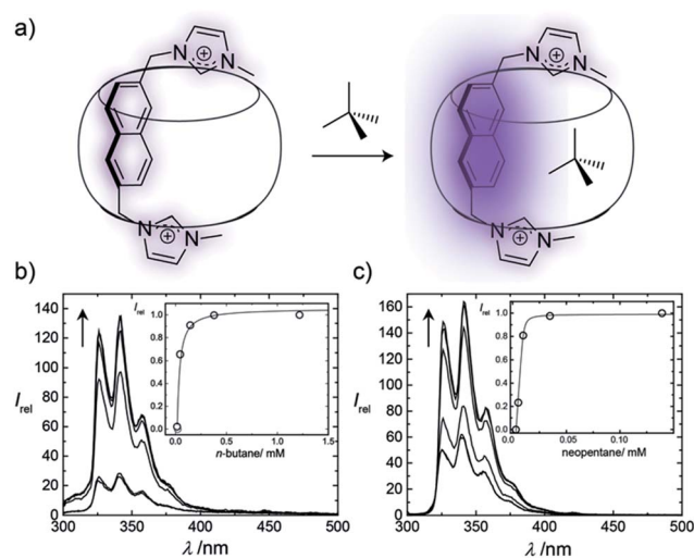
Fig. 3 (a) The encapsulation of a second guest within a Bis \cdot CB8 complex enhances the fluorescence of the first guest; changes in fluorescence can be directly correlated to the binding strength of the second guest. (b) and (c) Changes in fluorescence spectra for Bis2 \cdot CB8 complexes, plotted versus wavelength and second guest concentration (inset) for (b) n -butane and (c) neopentane.
