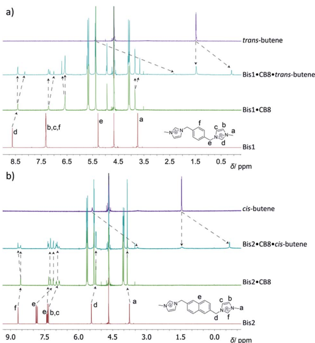
Fig. 2 ^1\text{H} NMR spectra for the binding of (a) trans -butene to the Bis1 \cdot CB8 complex and (b) cis -butene to Bis2 \cdot CB8, in \text{D}_2\text{O} .
