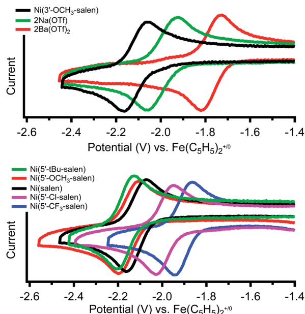
Fig. 2 Cyclic voltammograms of the reversible Ni(II/I) redox couples of (top) Ni(3'-OCH 3 -salen) and 2M (M = Na + , Ba 2+ ) and (bottom) Ni(5'-R-salen) where (R = CF 3 , Cl, tBu, OCH 3 ) in 0.1 M tetrabutylammonium hexafluorophosphate in dimethylformamide under N 2 at a scan rate of 1 V s -1 .
