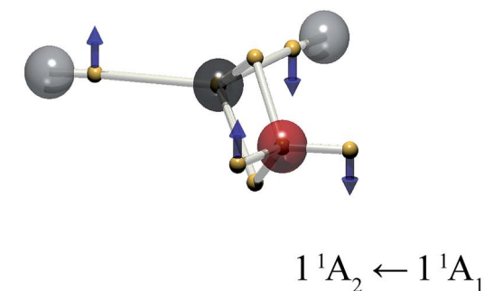
Fig. 4 The electron positions for the mid-point of the vibration, \bar{x} = (\bar{x}_i + \bar{x}_j)/2 , and the displacement vector x_{fi} for the wavefunction mixed between the 1^1A_1 (ground), and 1^1A_2 , 2^1A_1 and 1^1B_1 excited states of formaldehyde. The vector length is doubled for clarity.
