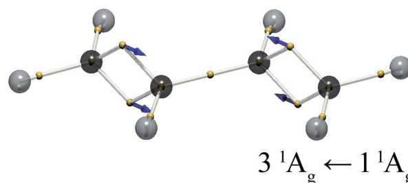
Fig. 5 The electron positions for the mid-point of the vibration, \bar{x} = (\bar{x}_i + \bar{x}_j)/2 , and the displacement vectors x_{fi} , for the 1^1B_u \leftarrow 1^1A_g and 3^1A_g \leftarrow 1^1A_g transitions of trans -butadiene. The vector length is doubled for clarity.
