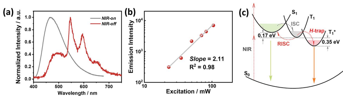
Fig. 5 (a) Two-photon-induced steady-state emission and delayed emission (delay = 8 ms) of o -Cz excited with a 808 nm femtosecond laser; (b) plots of emission intensity varying with input laser density (collected at 542 nm); (c) proposed mechanism of the two-photon induced ultralong phosphorescence in o -Cz. The energy levels are obtained with experimental spectra of the crystalline o -Cz.
