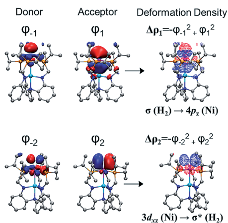
Fig. 4 The two dominant NOCV pairs in 3-H 2 and their associated deformation densities (Δρ 1 , top right; Δρ 2 , bottom right; contour iso-value = 0.04 a.u.). The colors of the deformation densities indicate the flow of electrons, from red to blue, involved in the Ni-H 2 interaction.
